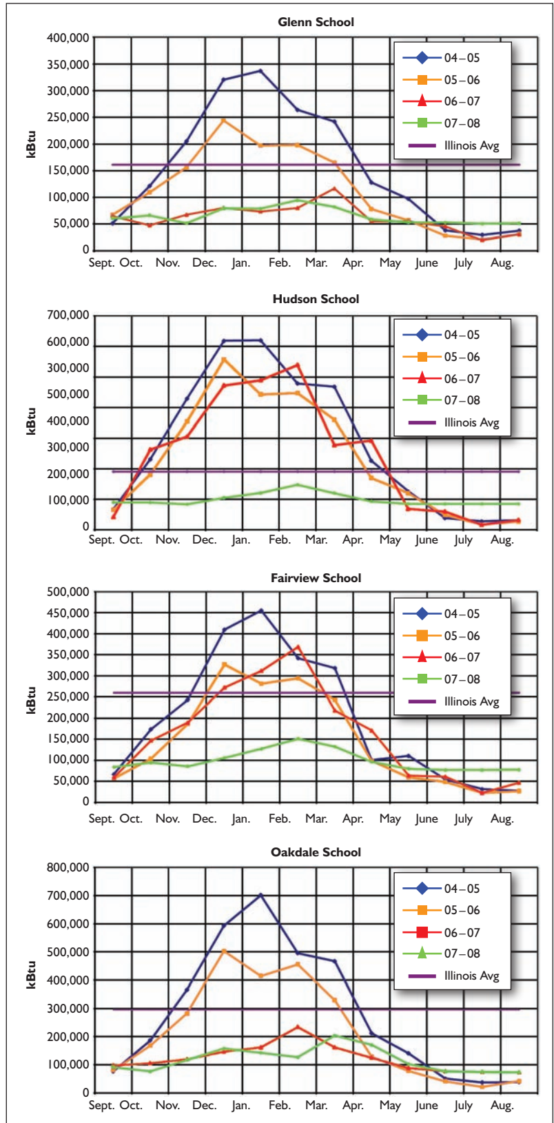
Figure 11: Energy use history of one-pipe schools.
