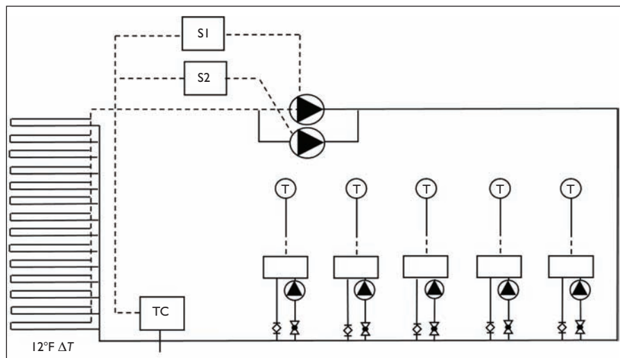
Figure 2: One-pipe system.
