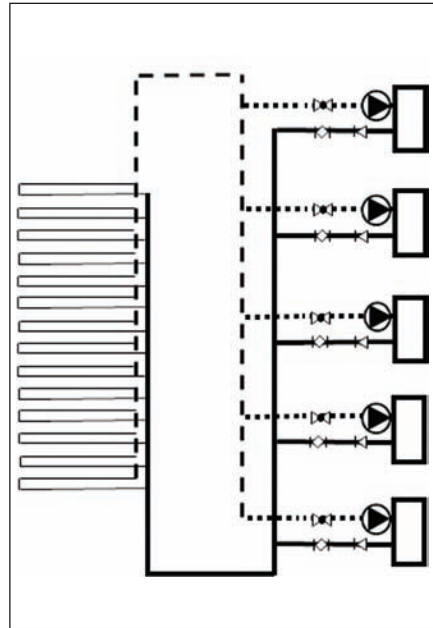
Figure 4: Subcentral GCHP.
