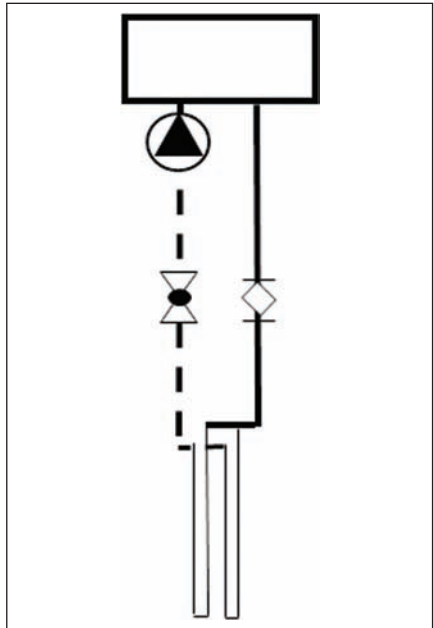
Figure 3: Simple GCHP.
