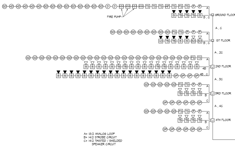
PAQUIN TOWERS 01 FIRE ALARM RISER DIAGRAM SCALE: NONE
